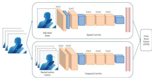
Fig. 3. Framework [10]
