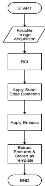
Fig. 9. Flow Chart for Enrollment
