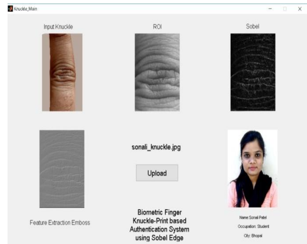
Fig. 7. Proposed GUI
