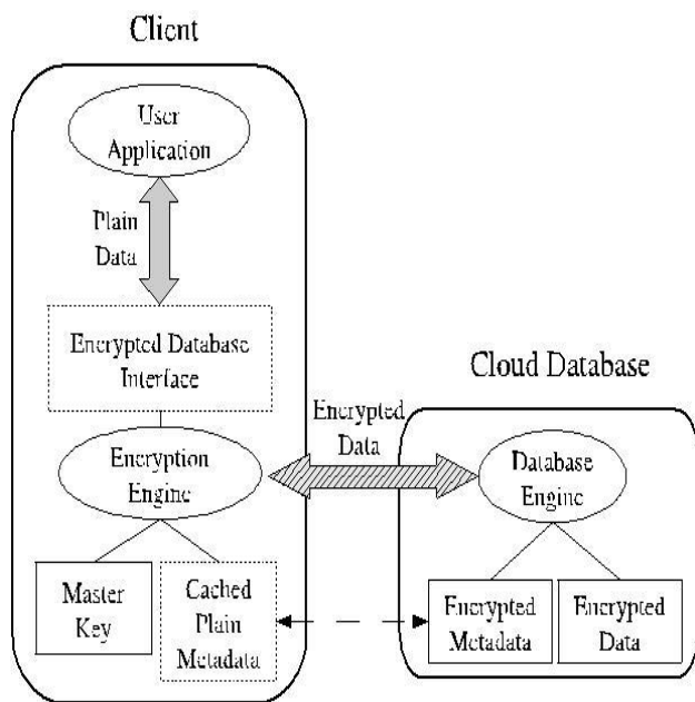
Fig. 3. Encrypted Cloud Database [14]
