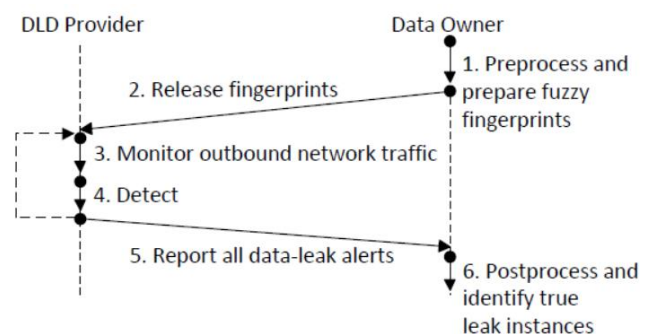
Fig. 4. Privacy Preserving Data Leak Detection Model [18]
