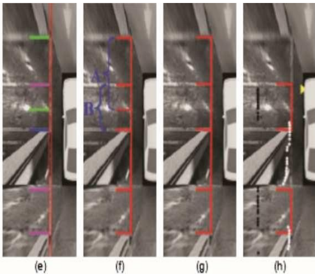
Fig. 9. Parking Slot Occupancy Detection (e) Separating lines. (f) Initial parking slots. (g) Non-overlapped parking slots. (h) Vacant parking slots.
