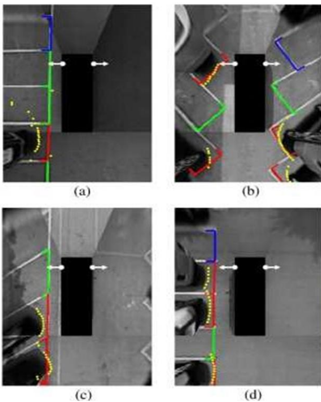
Fig. 6. Parking Slot Occupancy Classification in case of (a) TT-slots, (b) TL-slots, (c) YY-slots, and (d) II-slots
