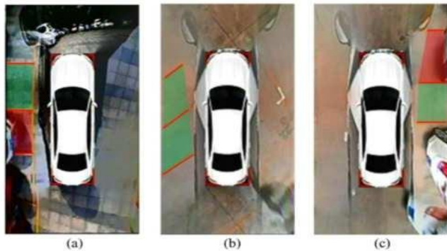
Fig. 14. Experiments Results of Typical Parking Slot. (A) Rectangular Type. (B) Slated Rectangular Type. (C) Open Rectangular Types
