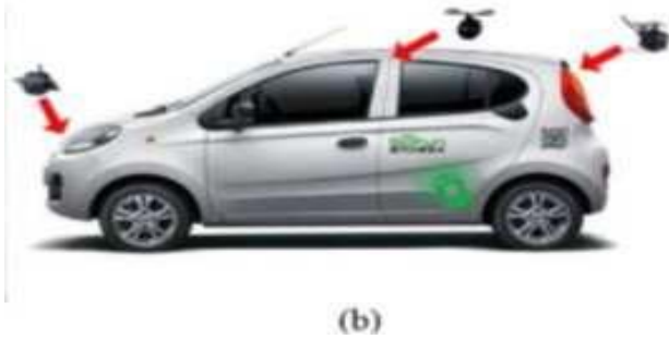
Fig. 13. (b) Location of cameras in the AVM system
