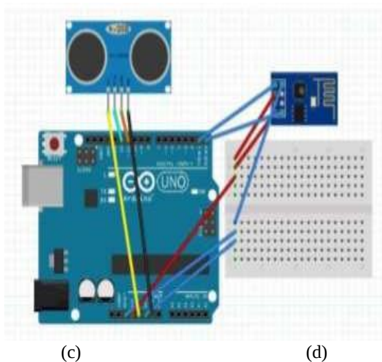
Fig. 10. Arduino Uno Board With Ultrasonic Sensors' Circuitry
