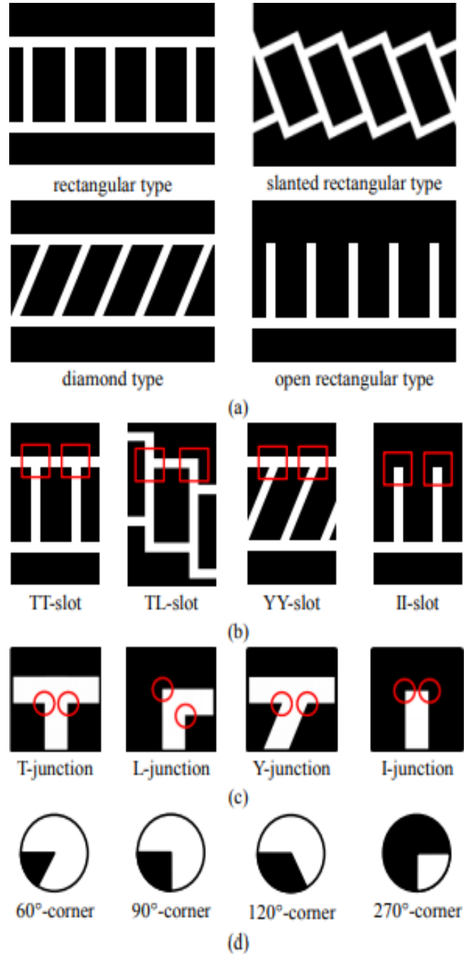
Fig. 5. Hierarchical tree structure of parking slot markings. (a) Parking slot markings. (b) Slots. (c) Junctions. (d) Corners.
