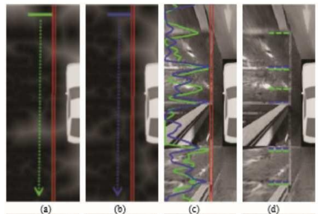
Fig. 8. Parking Slot Occupancy Detection (a) Positive DT image. (b) Negative DT image. (c) Chamfer matching scores. (d) Positive and negative lines.
